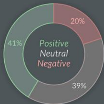
Sentiment
